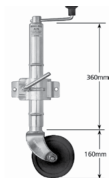
6" MULTI FIT SWING UP JOCKEY WHEEL
