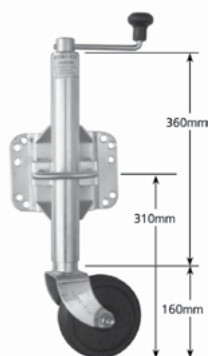
6" MULTI FIT SWING UP JOCKEY WHEEL
