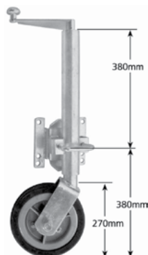
10" HEAVY DUTY GALVANISED MULTI FIT SWING UP JOCKEY WHEEL
