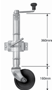
6" JOCKEY WHEEL WITH CLAMP
