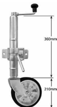
8" LONG REACH JOCKEY WHEEL WITH HEAVY DUTY HANDLE (CLAMP SOLD SEPERATLEY)
