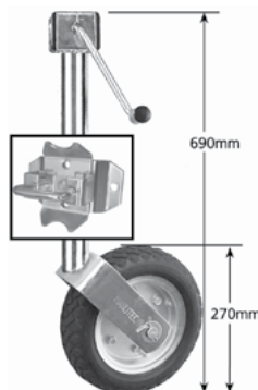
10" SIDE WIND SOLID PNEUMATIC JOCKEY WHEEL LOOSE SWING UP BRKT
