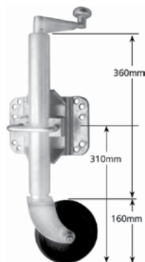
6" SWING UP JOCKEY WHEEL ECONOMY
