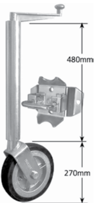
10" H/DUTY SWING UP JOCKEY WHEEL
