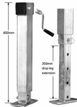
H/DUTY SIDE WIND 2 STAGE DROP LEG ONLY (LOOSE HANDLE)
