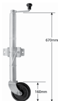
6" LONG REACH JOCKEY WHEEL WITH CLAMP
