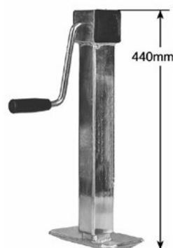
LIGHT DUTY SIDE WIND STAND ONLY
