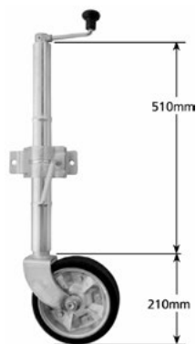
8" LONG REACH JOCKEY WHEEL WITH CLAMP
