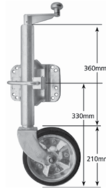
8" HEAVY DUTY MULTIFIT SWING UP JOCKEY WHEEL
