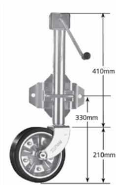
8" SWING UP JOCKEY WHEEL
