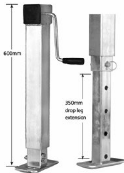
H/DUTY SIDE WIND 2 STAGE DROP LEG ONLY (FIXED HANDLE)
