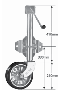
8" SIDE WIND SWING UP JOCKEY WHEEL
