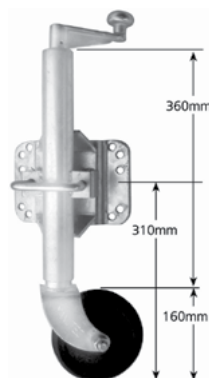
6" MULTI FIT SWING UP JOCKEY WHEEL
