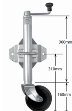
6" JOCKEY WHEEL WITH CLAMP
