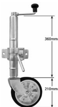
8" MULTIFIT SWING UP JOCKEY WHEEL
