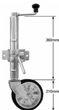
8" JOCKEY WHEEL WITH CLAMP
