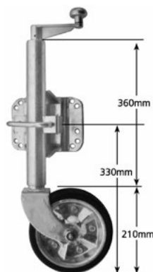
8" GALVANISED MULTIFIT SWING UP JOCKEY WHEEL
